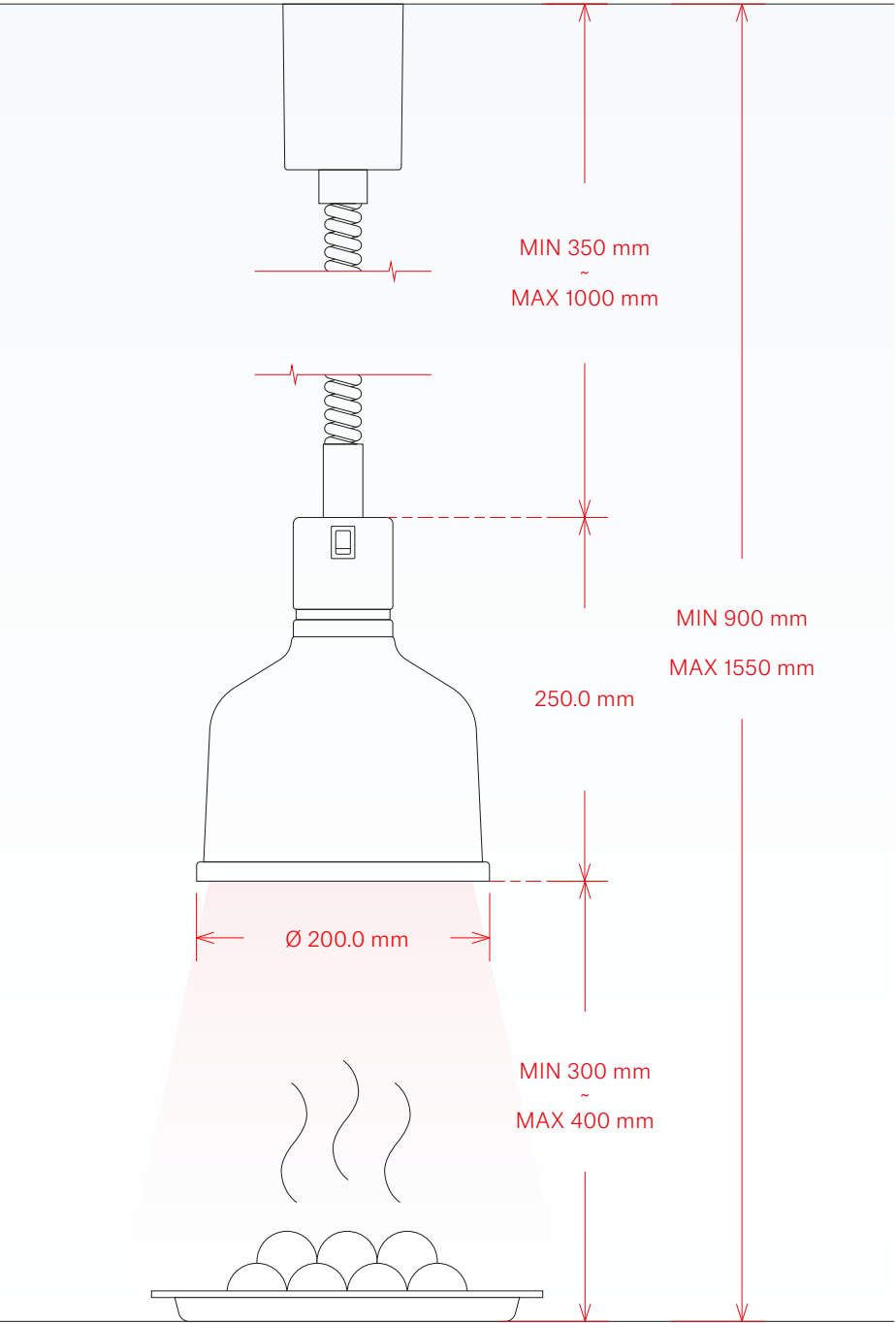
Short Cord
